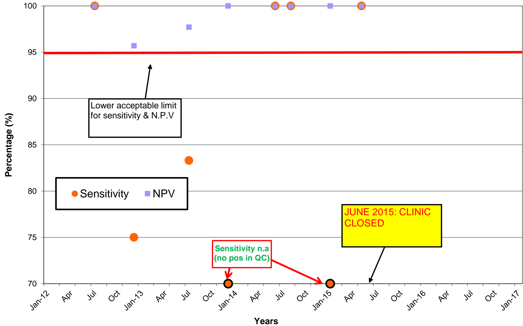
Sensitivity / NPV in S.M.R.U P.L.U CLINIC (Jan-2012 to May-2015)
