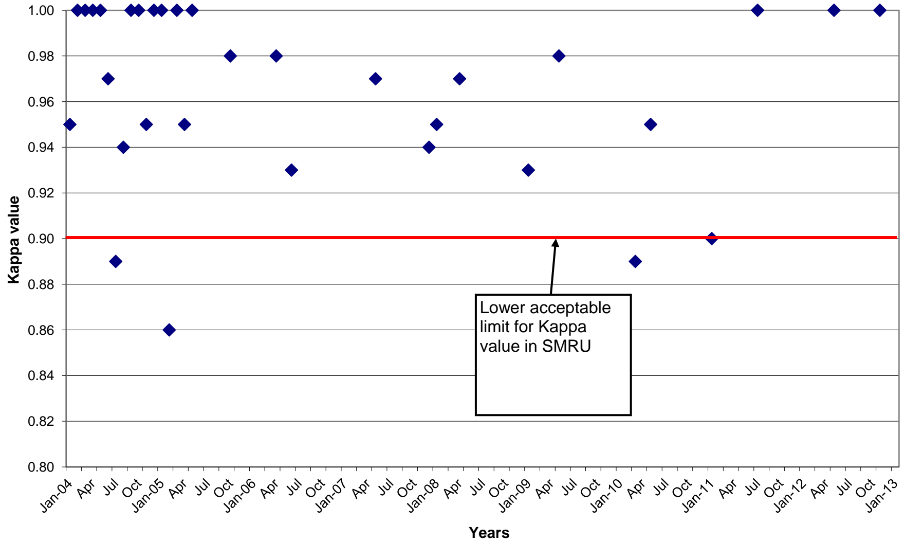
Kappa in S.M.R.U M.K.T CLINIC (Jan-2004 to Jan-2013)
