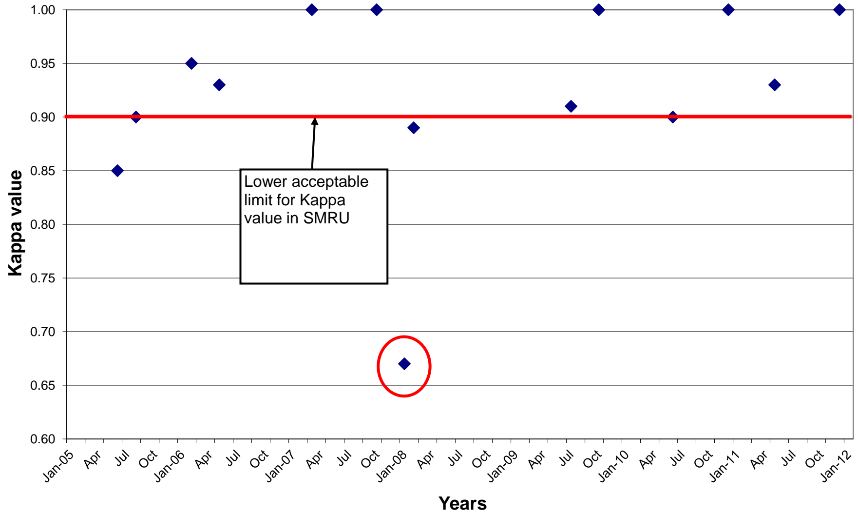
Kappa in S.M.R.U P.L.U CLINIC (Jan-2005 to Dec-2011)
