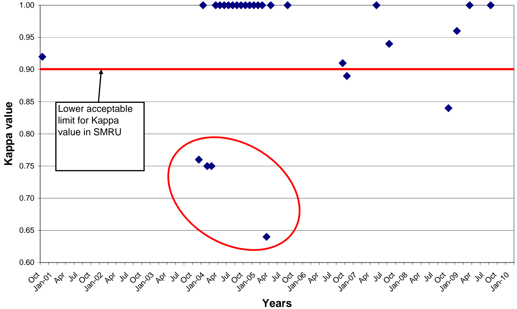
Kappa in S.M.R.U M.R.C CLINIC (Oct-2000 to Jan-2010)
