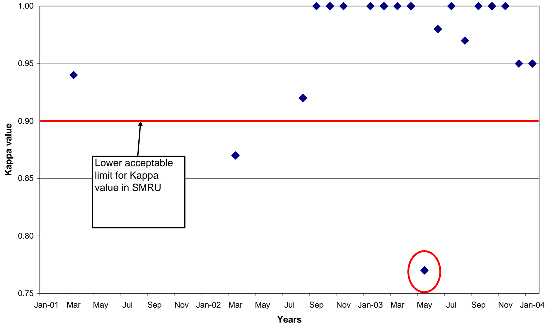
Kappa in S.M.R.U M.K.T CLINIC (Jan-2001 to Jan-2004)
